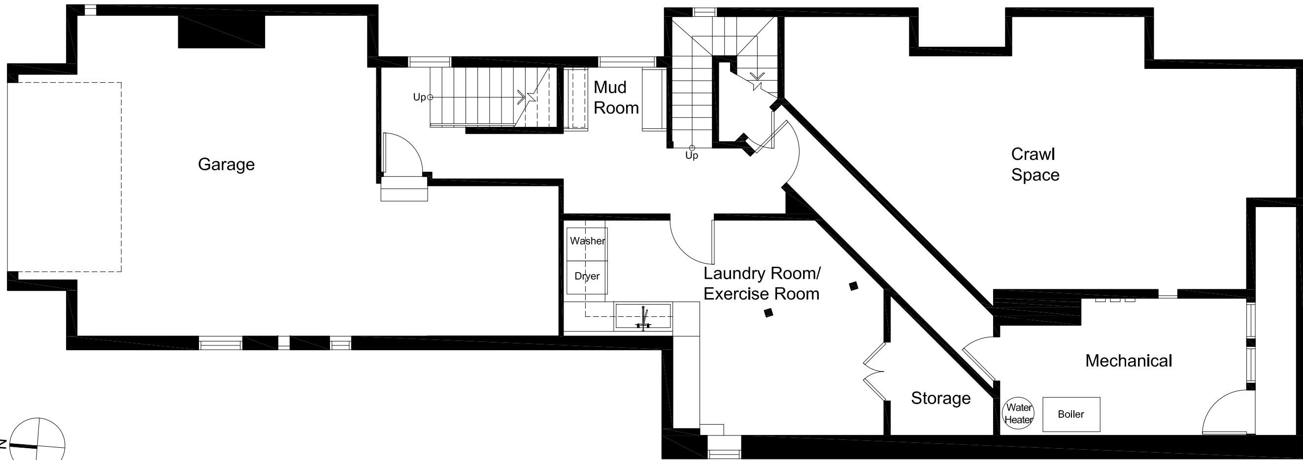
Basement Level Floor Plan
