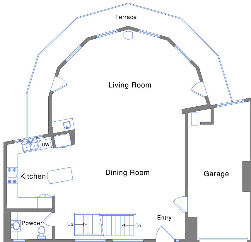
Third Floor
