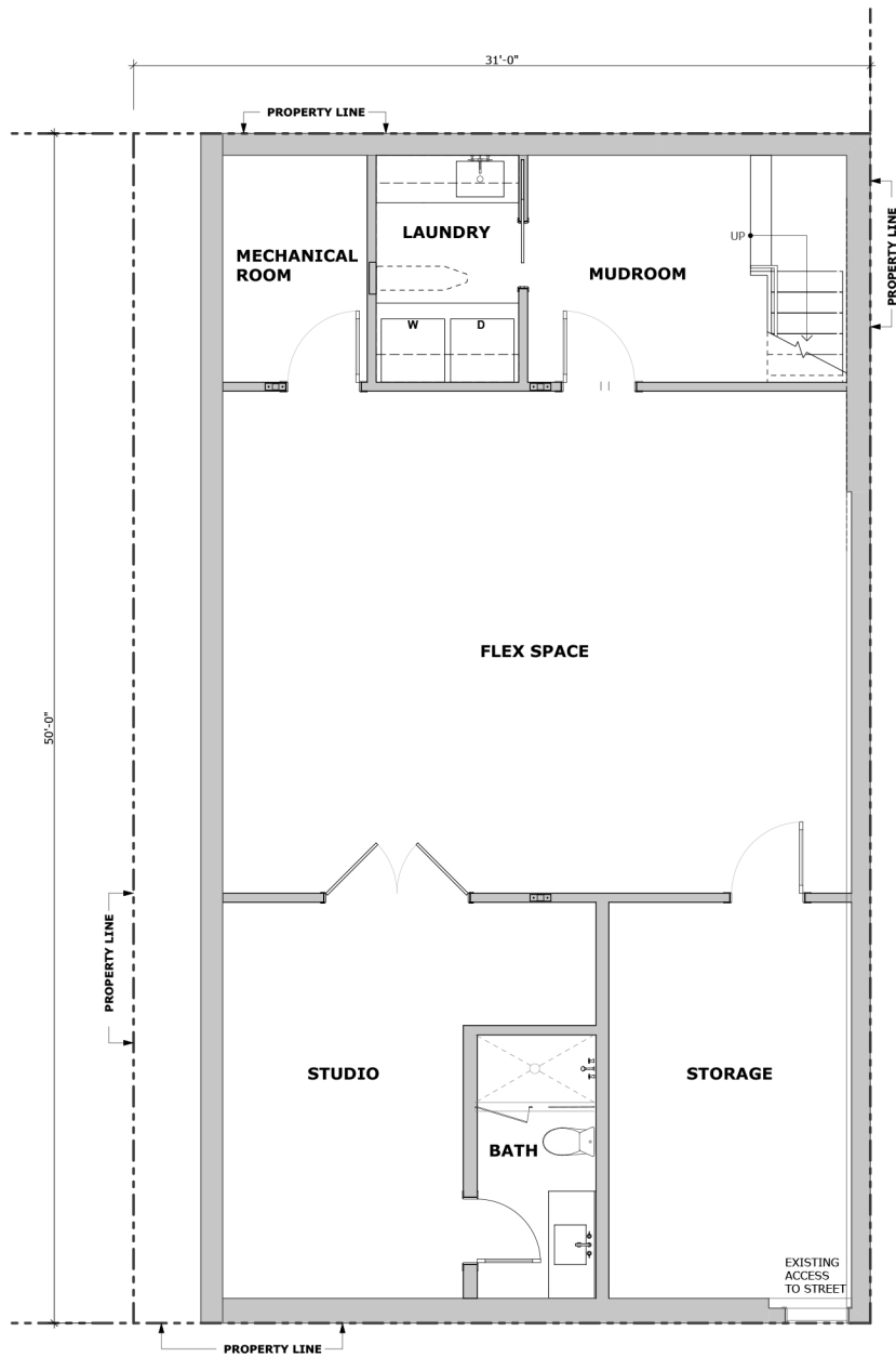
Proposed Basement Plan
