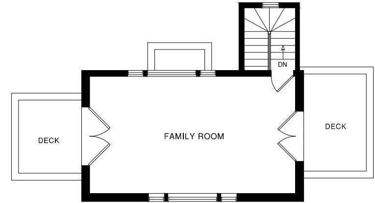
THIRD FLOOR
