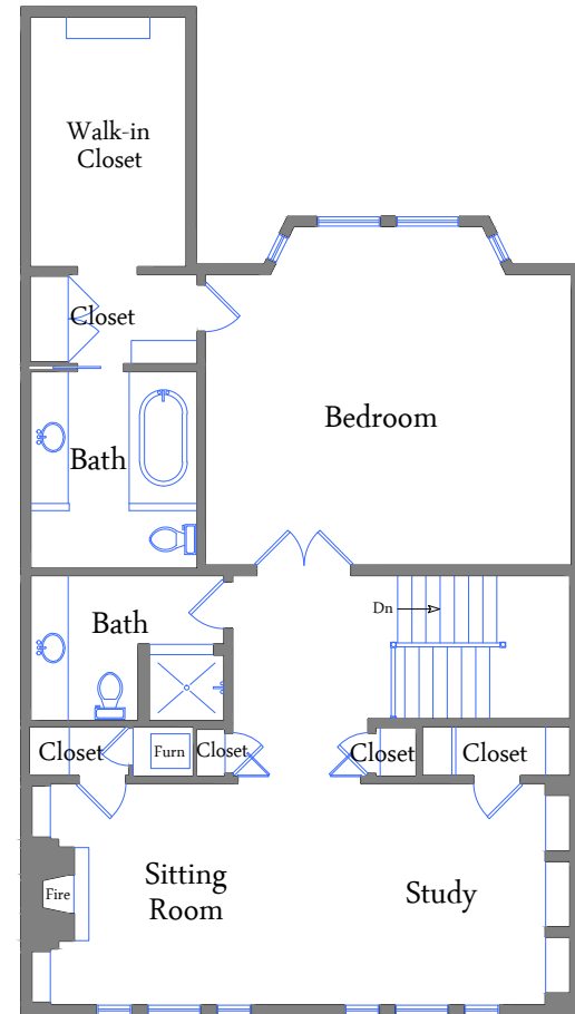
Third Level
