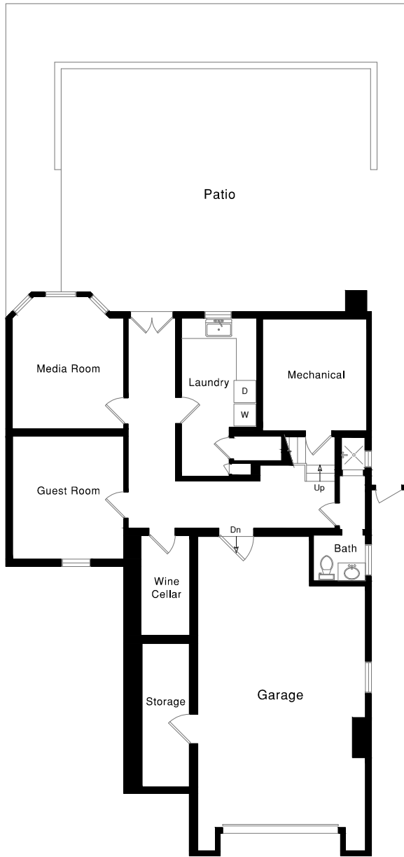
Lower Level
